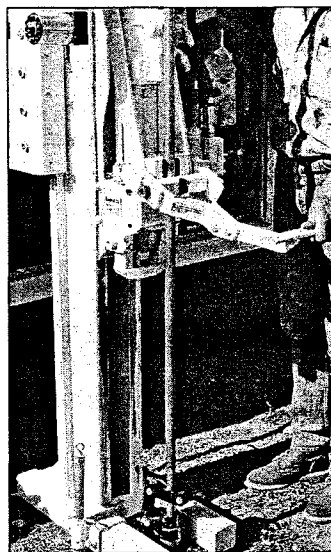
Figure 4.26. Raise the inner rod string using the probe hammer and a Rod Grip Pull System if rods are too heavy to lift by hand.
