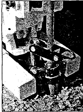
Figure 4.10. The DT21 Rod Clamp Assembly holds the inner rod string while adding or removing 1.0-inch rods.
