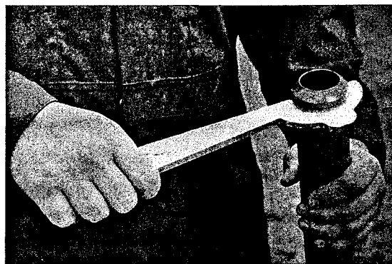
Figure 4.6. Tighten MC Cutting Shoe with MC Combination Wrench.
