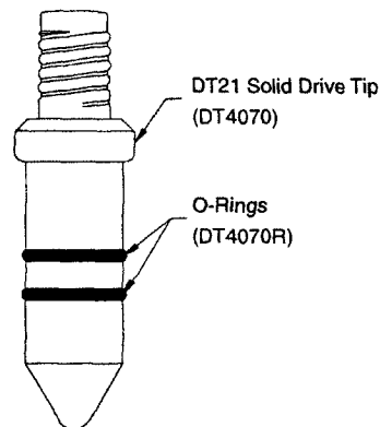
FIGURE 4.5 Solid Drive Point is Fitted with Two O-Rings
